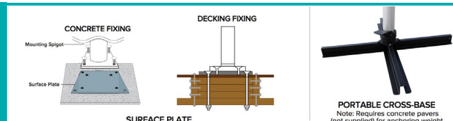
SURFACE PLATE
